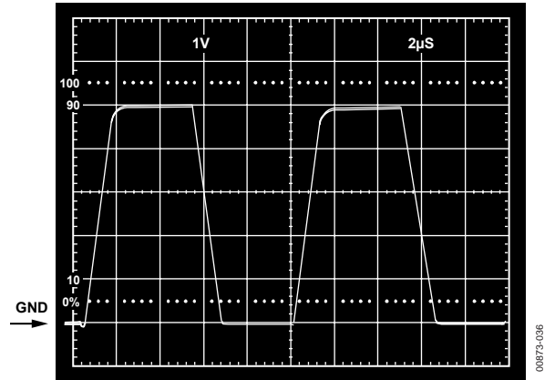
Figure 36. V_S = 5\text{ V}, 0\text{ V} ; Gain of Two Inverter Response to 2.5 V Step, Centered -1.25 V Below Ground
